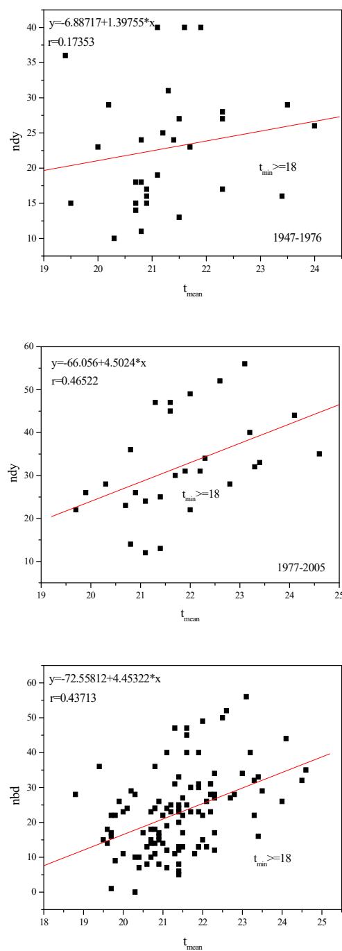
Fig. 5. Relationship between occurrence of minimum temperature \geq 18^\circ\text{C} and the mean summer temperature during the period 1888-2005 in Belgrade.
