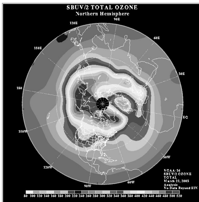
Fig. 6. Opening of the magnetospheric door on 21. 03. 2003 http://www.cpc.ncep.noaa.gov/products/stratosphere/sbu2to/gif_files/sbu2to_nh_latest.gif
