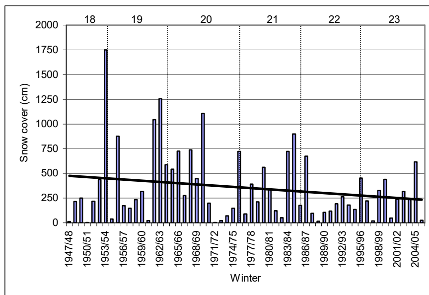
Figure 4 Seasonal snow cover (December, January and February) for 1948-2006 period. Solar cycle numbers are above.
