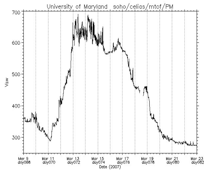
Picture 7. Solar wind velocity from CH260
