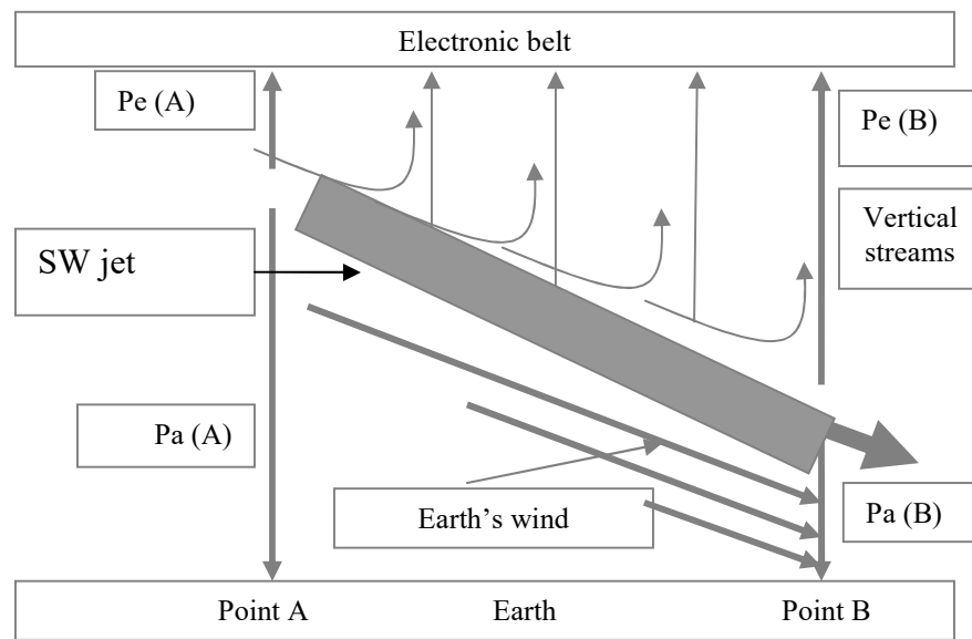
Fig. 9. The schematic review of the penetration of the SW jet into the atmosphere (Stevancevic, 2006).
